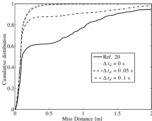
Fig. 6 Cumulative miss distance distributions with logic-based tuned estimators.
