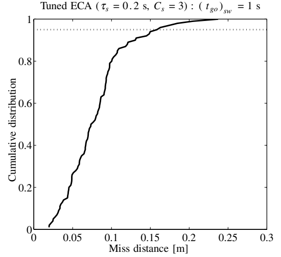
Fig. 4 Cumulative miss distance distribution of DGL/I with an ideally tuned estimator.
