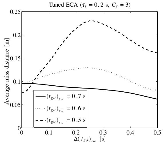
Fig. 5 Average miss distances with tuned estimators for bang-bang target maneuvers.
