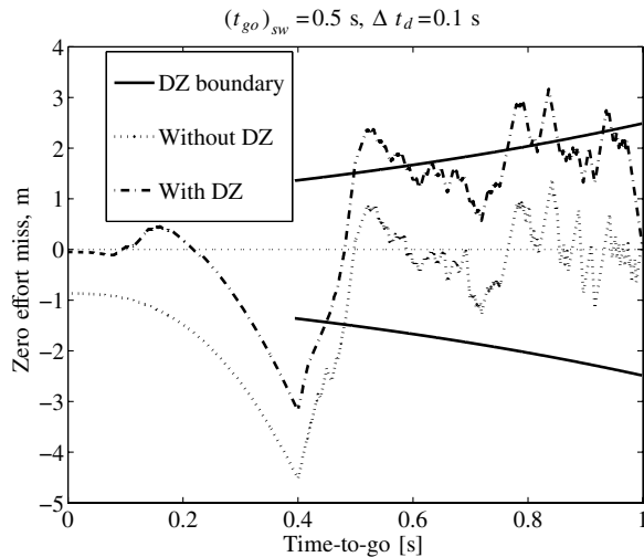
Fig. 8 The effect of time-varying dead zone.
