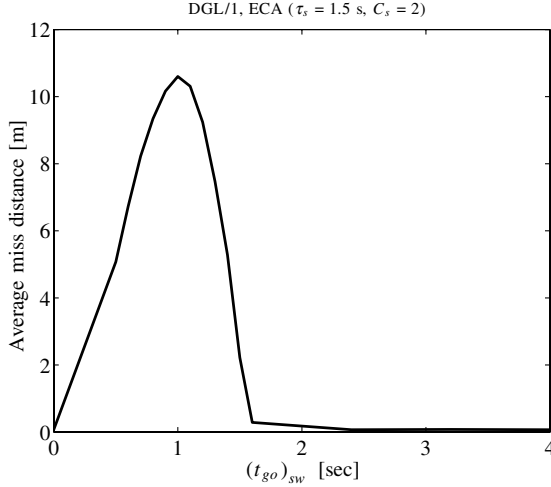
Fig. 2 Homing performance of DGL/1 against bang-bang target maneuvers.
