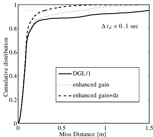
Fig. 9 Cumulative miss distance distributions with guidance law modifications.
