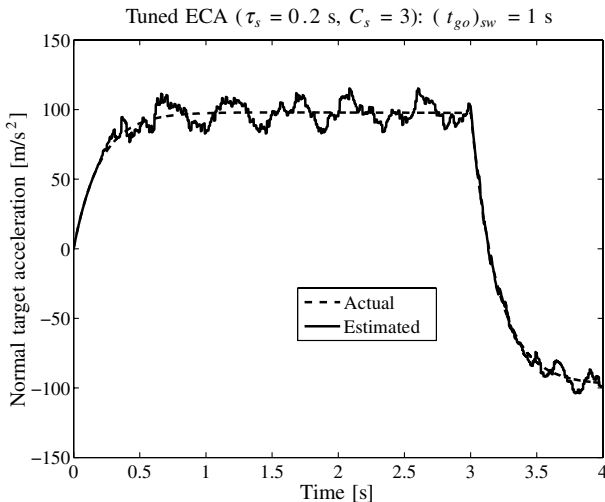
Fig. 3 Target acceleration estimation performance of an ideally tuned estimator.
