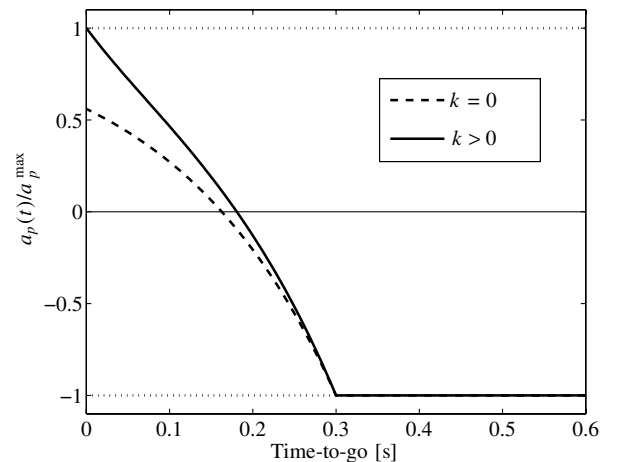
Fig. 7 The effect of command gain enhancement.
